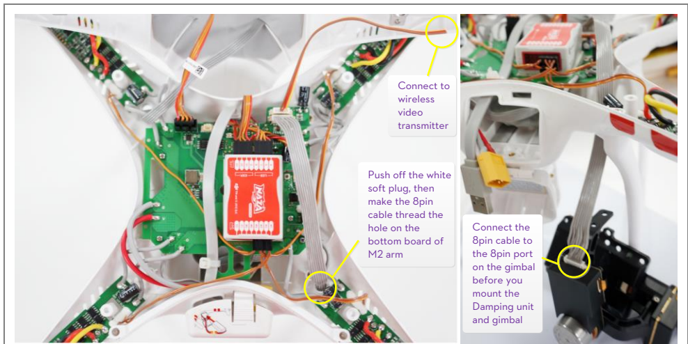
Fig.6 Final connections
