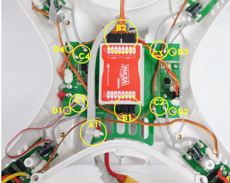
Fig.2 Disassemble items
